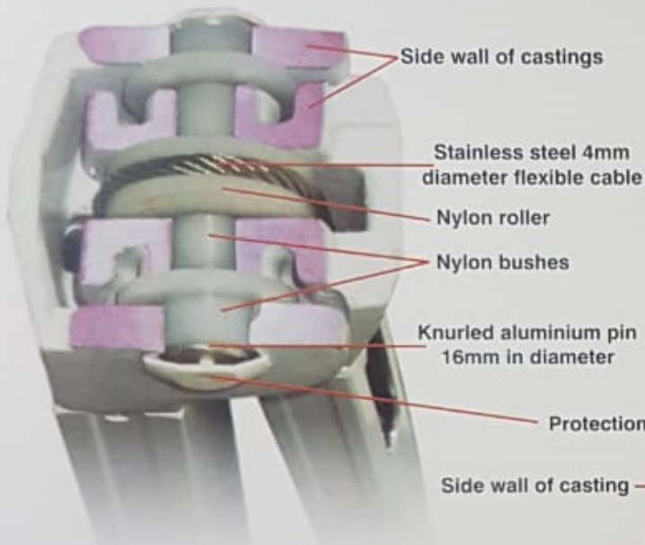
CUT AWAY SECTION OF ELBOW CASTINGS
