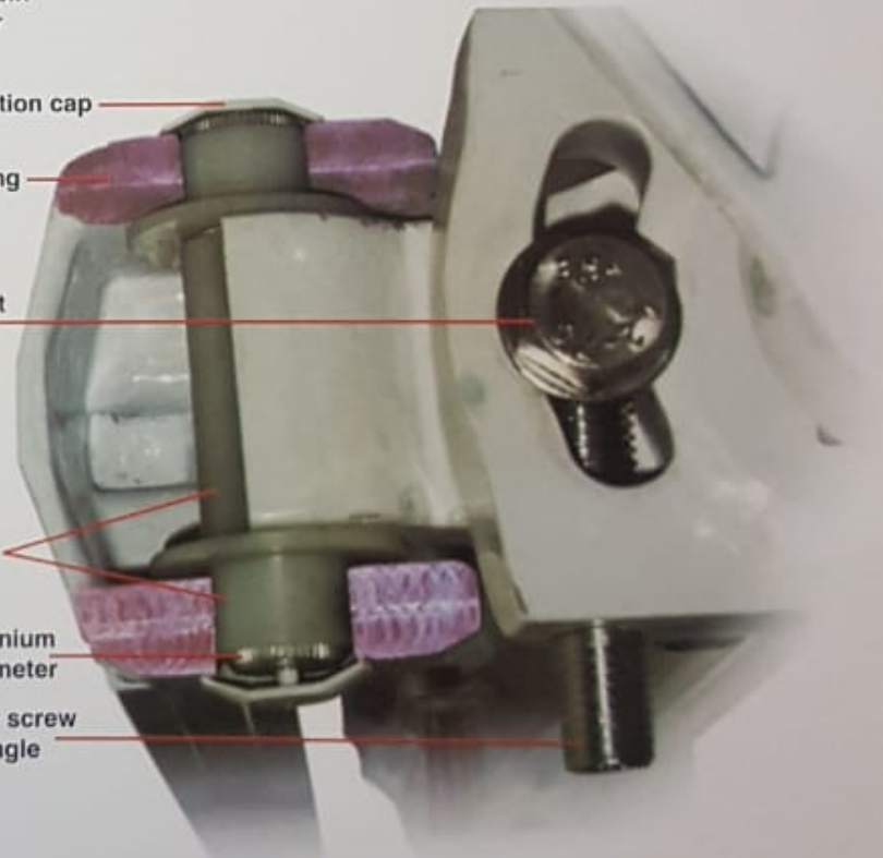
CUT AWAY SECTION OF SHOULDER CASTINGS AND ANGLE ADJUSTMENT
